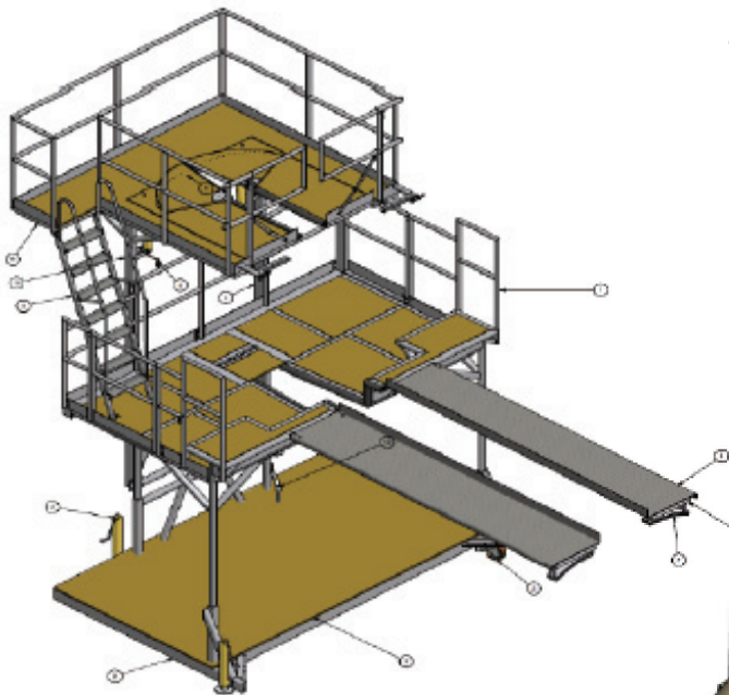
BAE Systems Typhoon / Eurofighter fin / rear fuselage access staging
